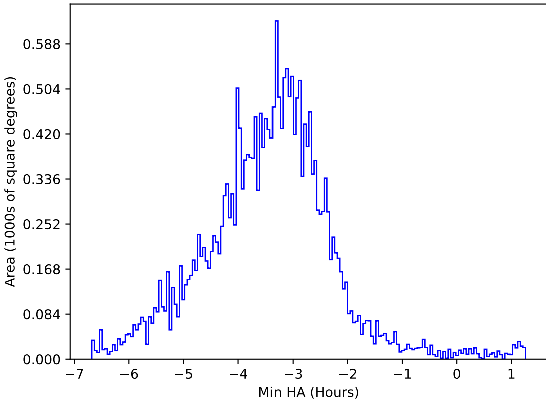
too_elab_r8_d3_griz_v3.4_10yrs All sky y band: Min HA
