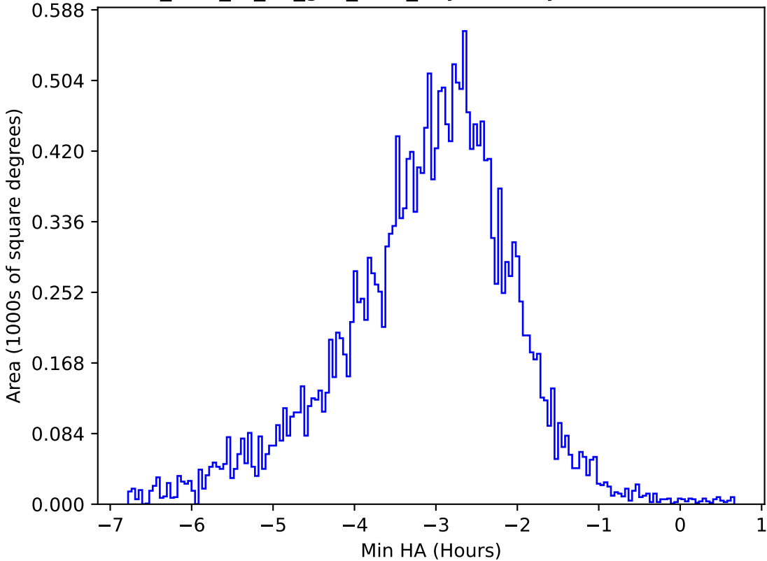
too_elab_r8_d3_griz_v3.4_10yrs All sky u band: Min HA
