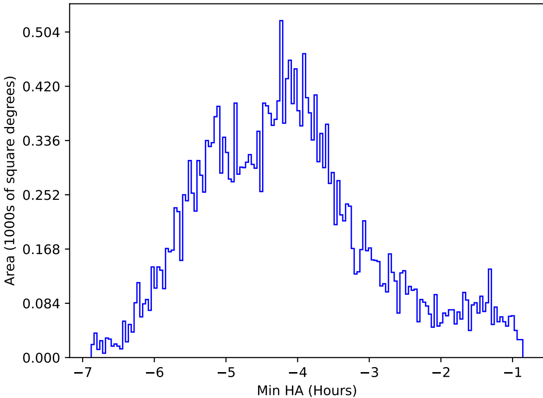
too_elab_r8_d3_griz_v3.4_10yrs All sky r band: Min HA
