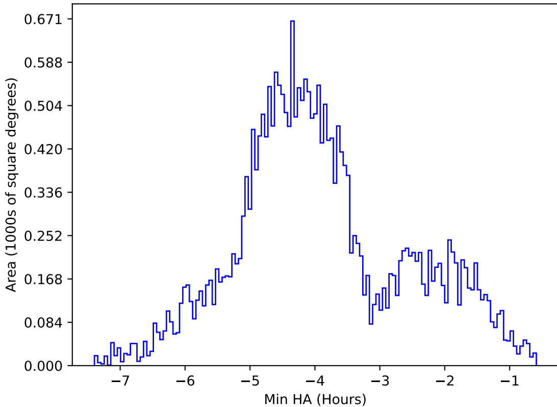
too_elab_r8_d3_griz_v3.4_10yrs All sky g band: Min HA
