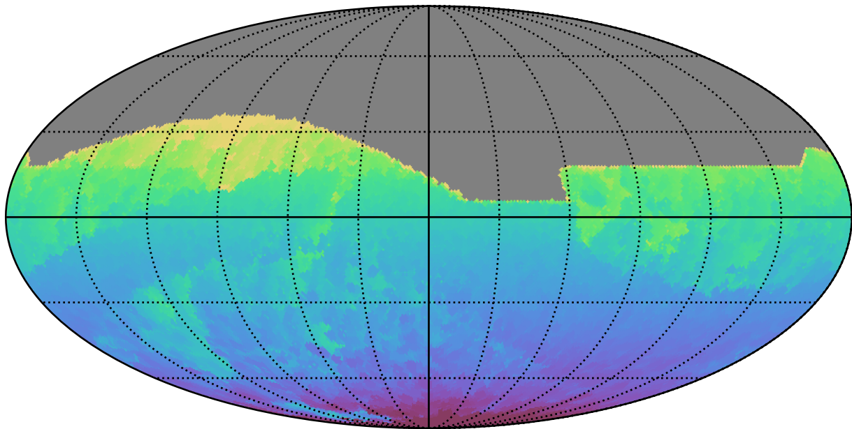
too_elab_r8_d3_griz_v3.4_10yrs All sky all bands: Min HA
