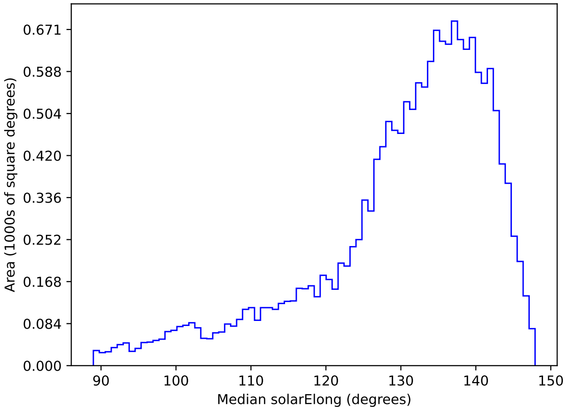
too_elab_r8_d3_griz_v3.4_10yrs WFD y band: Median solarElong
