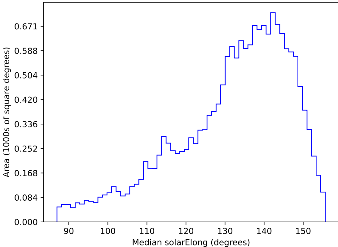
too_elab_r8_d3_griz_v3.4_10yrs WFD u band: Median solarElong
