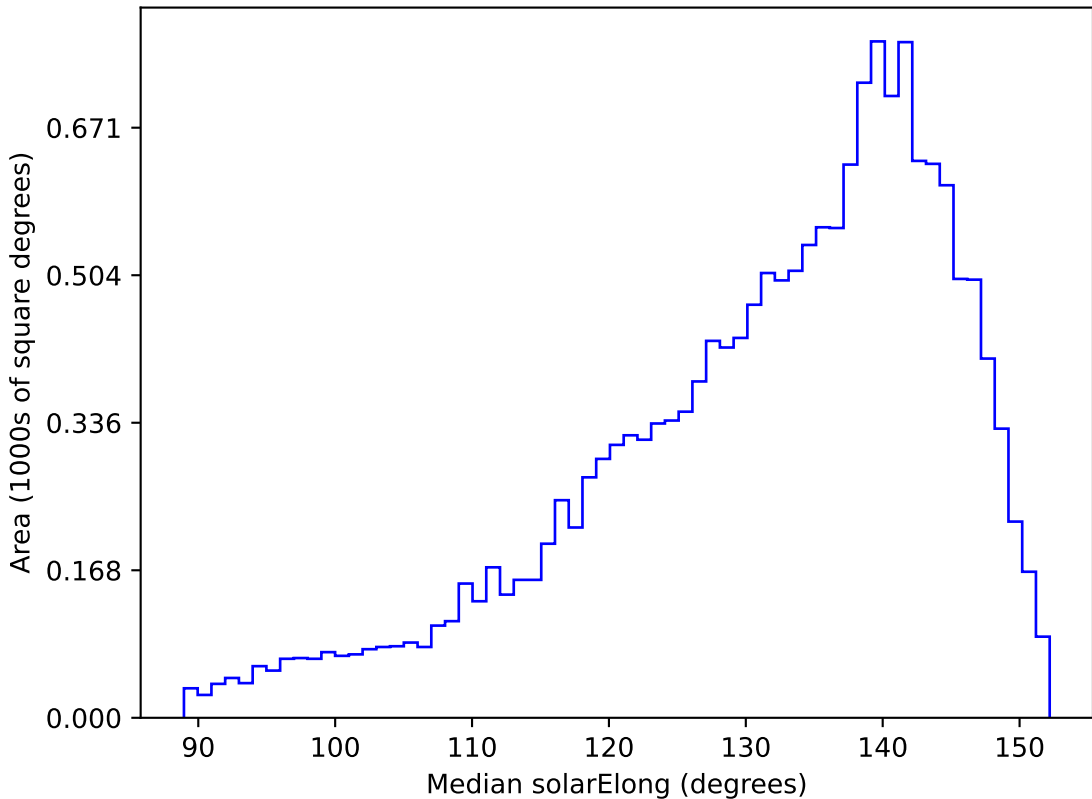
too_elab_r8_d3_griz_v3.4_10yrs WFD g band: Median solarElong
