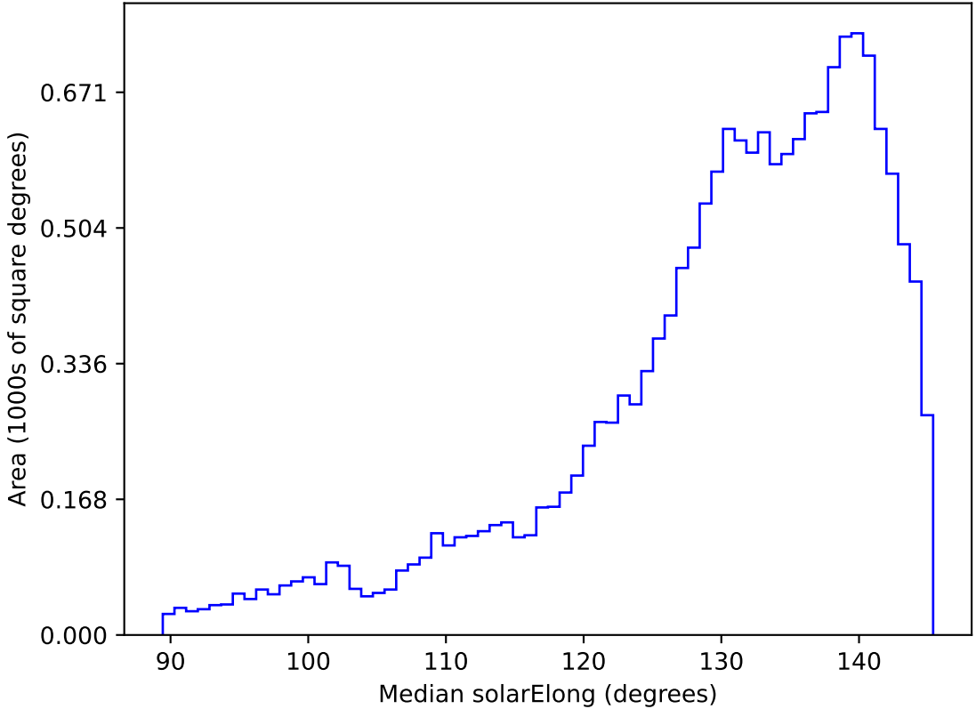
too_elab_r8_d3_griz_v3.4_10yrs WFD all bands: Median solarElong
