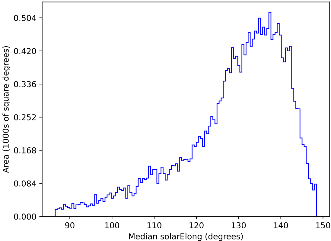
too_elab_r8_d3_griz_v3.4_10yrs All sky y band: Median solarElong
