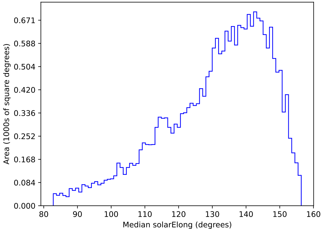
too_elab_r8_d3_griz_v3.4_10yrs All sky u band: Median solarElong
