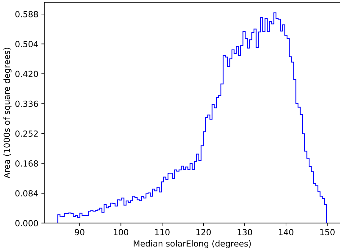
too_elab_r8_d3_griz_v3.4_10yrs All sky i band: Median solarElong
