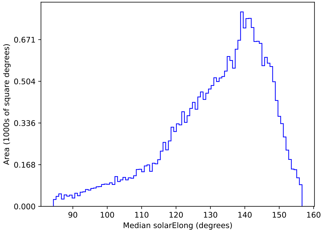
too_elab_r8_d3_griz_v3.4_10yrs All sky g band: Median solarElong
