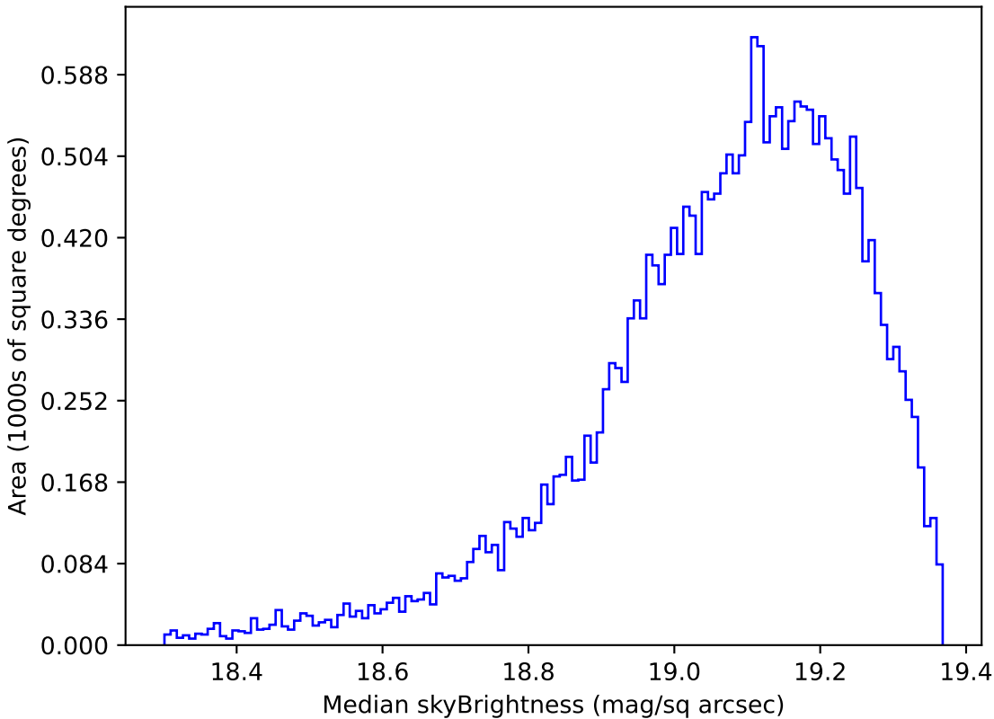
too_elab_r8_d3_griz_v3.4_10yrs Yr 1 z band: Median skyBrightness
