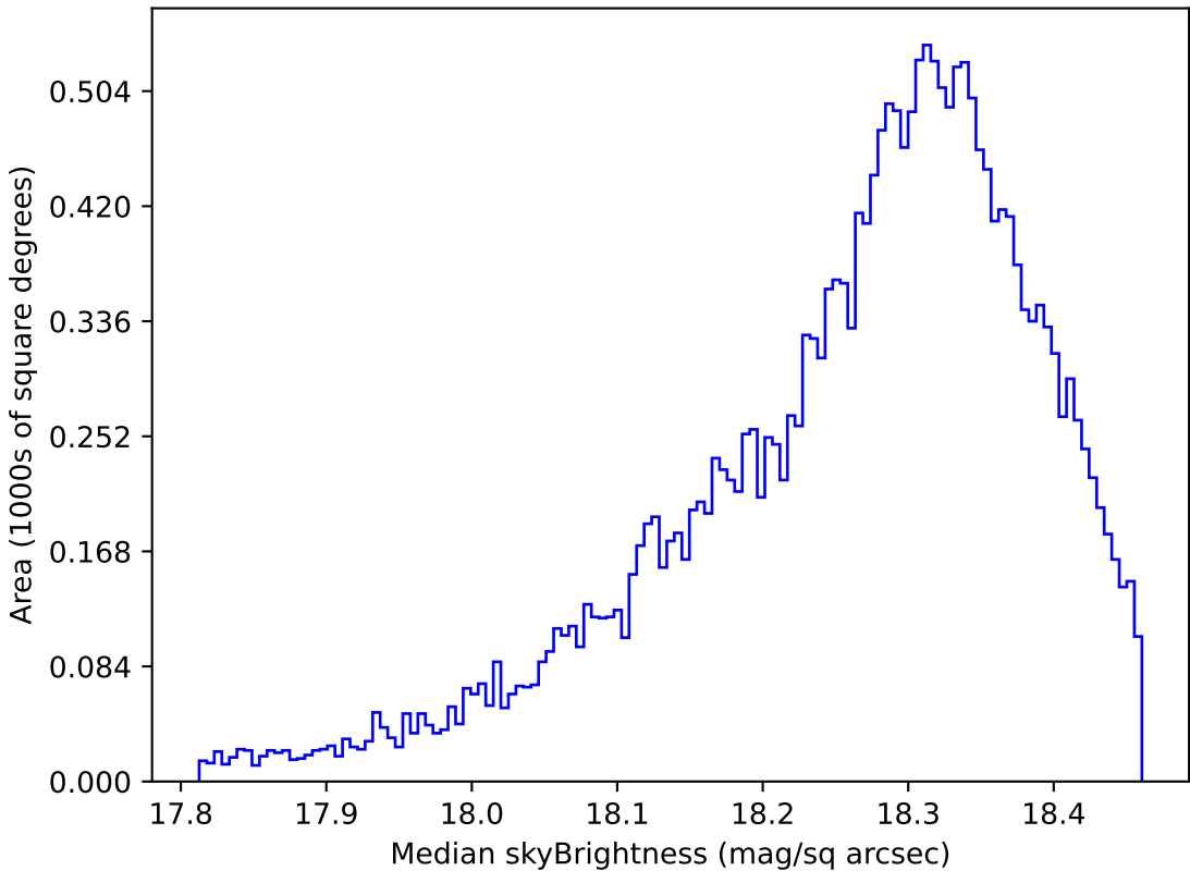
too_elab_r8_d3_griz_v3.4_10yrs Yr 1 y band: Median skyBrightness
