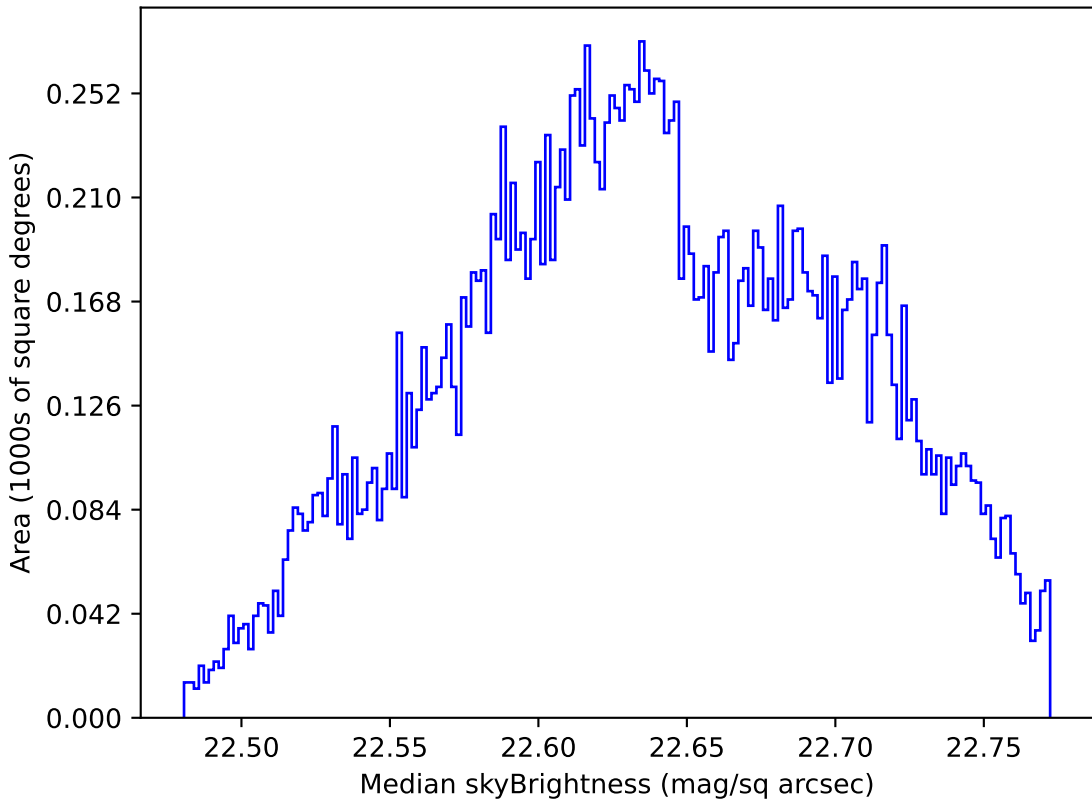
too_elab_r8_d3_griz_v3.4_10yrs Yr 1 u band: Median skyBrightness
