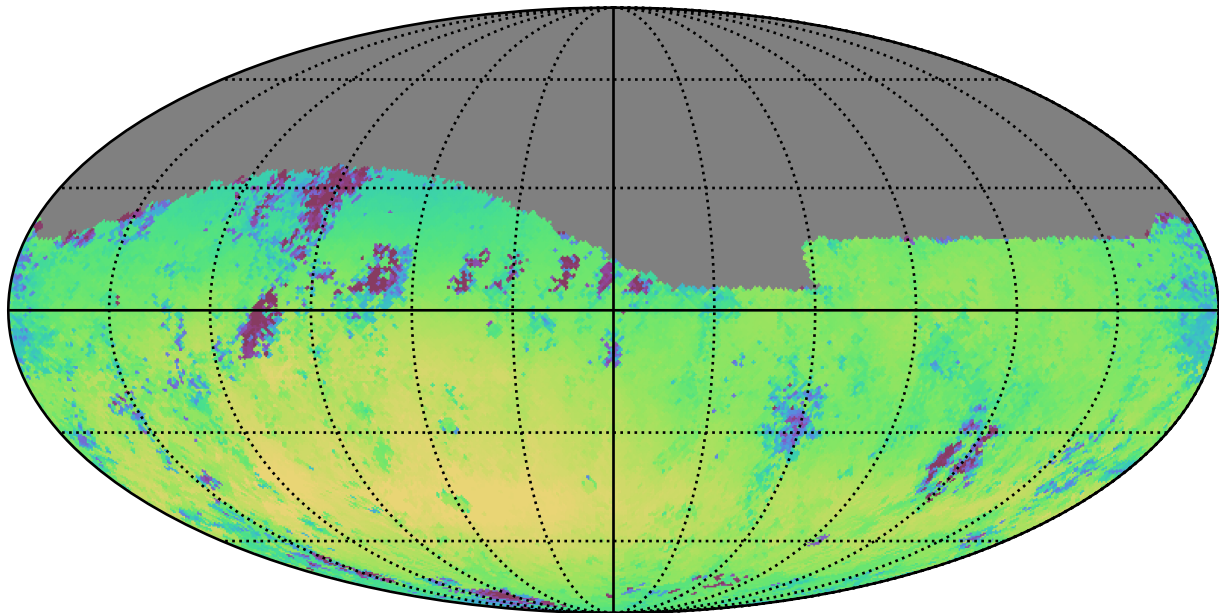
too_elab_r8_d3_griz_v3.4_10yrs Yr 1 r band: Median skyBrightness
