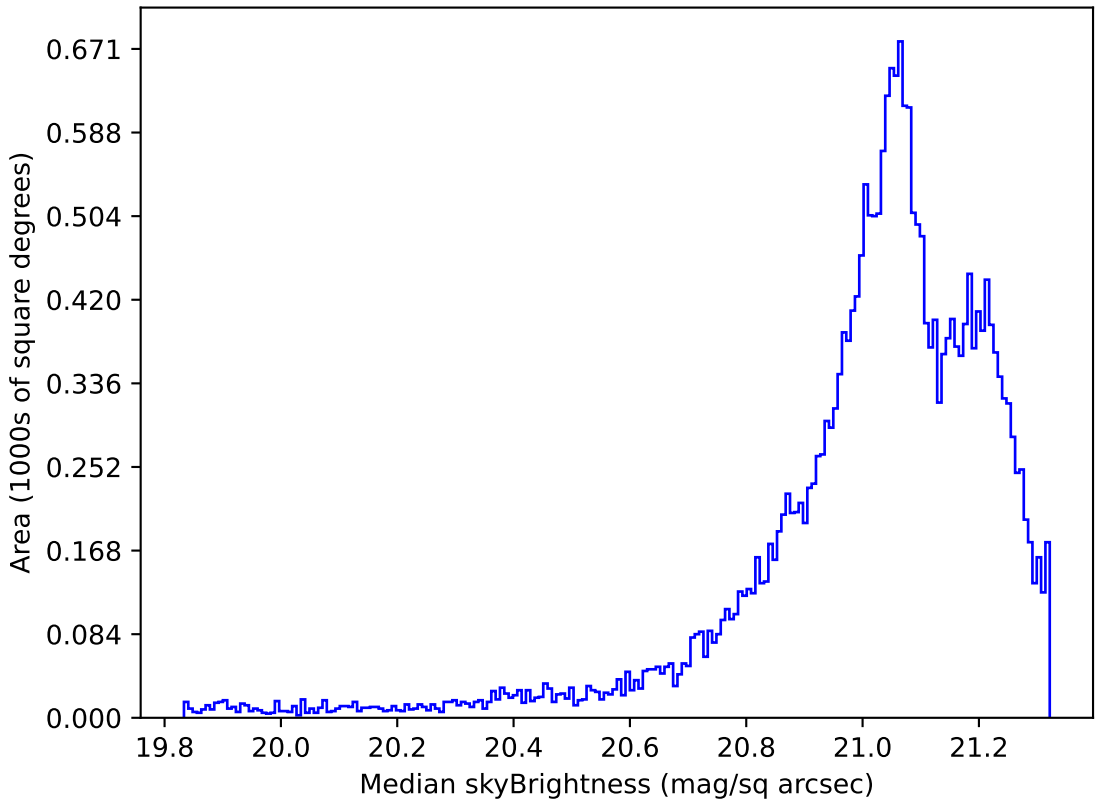
too_elab_r8_d3_griz_v3.4_10yrs Yr 1 r band: Median skyBrightness
