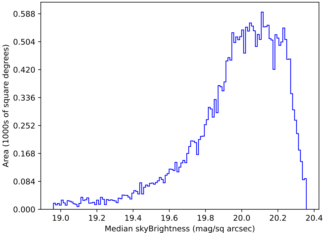
too_elab_r8_d3_griz_v3.4_10yrs Yr 1 i band: Median skyBrightness
