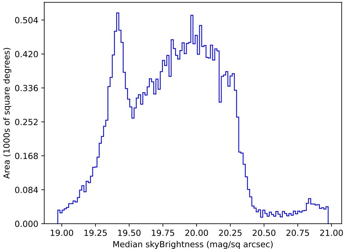
too_elab_r8_d3_griz_v3.4_10yrs Yr 1 all bands: Median skyBrightness
