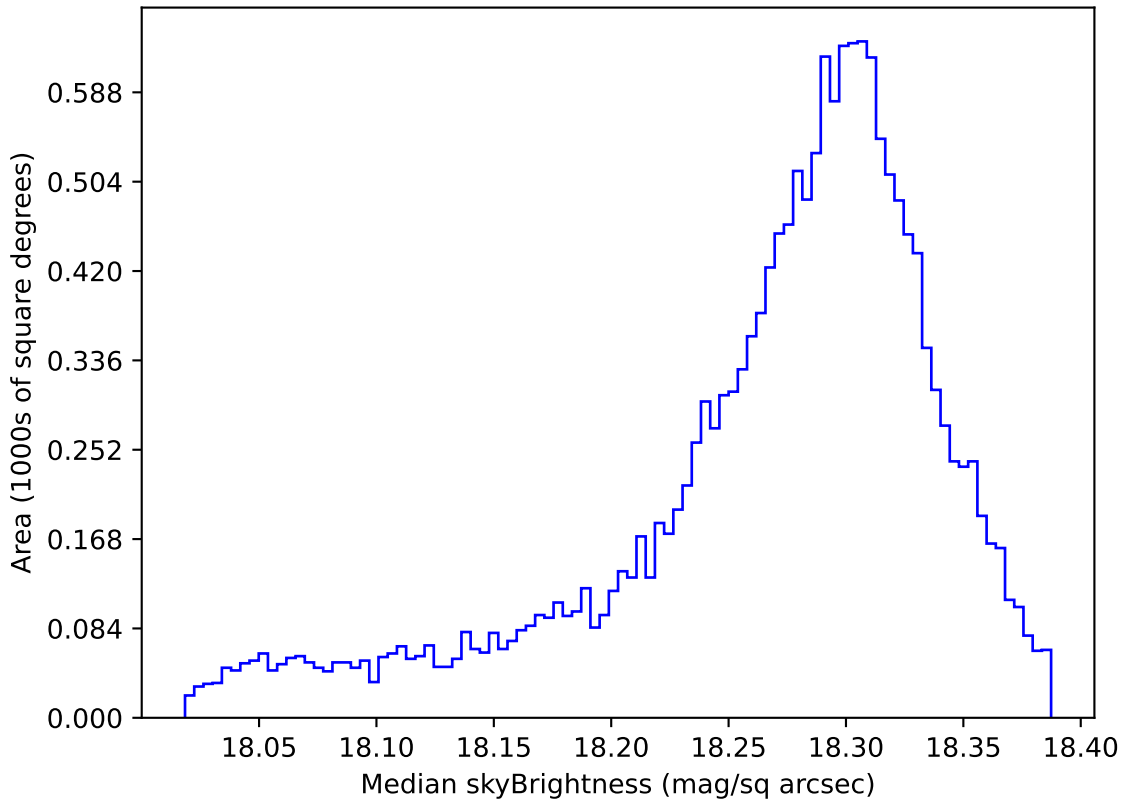
too_elab_r8_d3_griz_v3.4_10yrs WFD y band: Median skyBrightness
