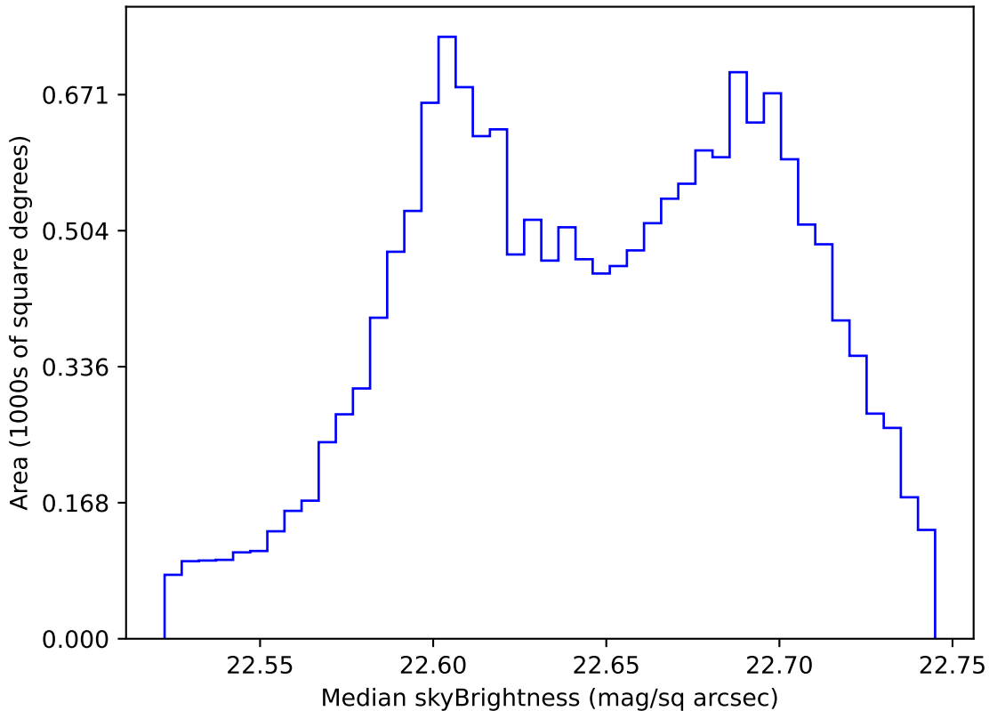
too_elab_r8_d3_griz_v3.4_10yrs WFD u band: Median skyBrightness
