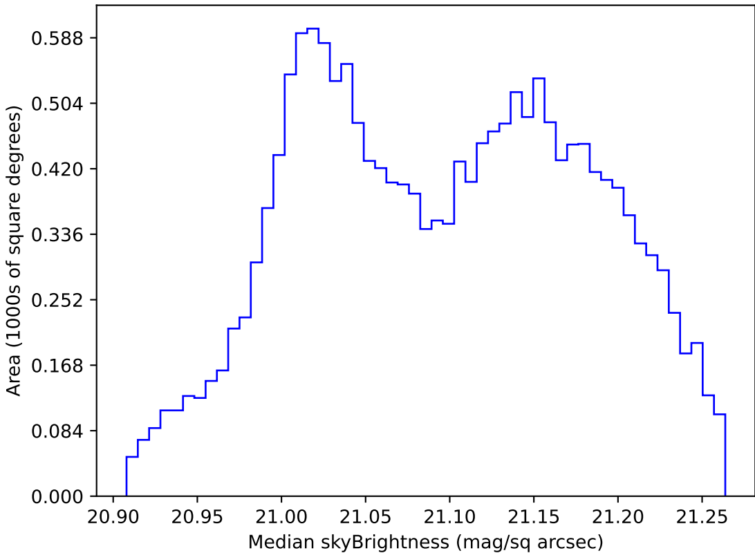
too_elab_r8_d3_griz_v3.4_10yrs WFD r band: Median skyBrightness
