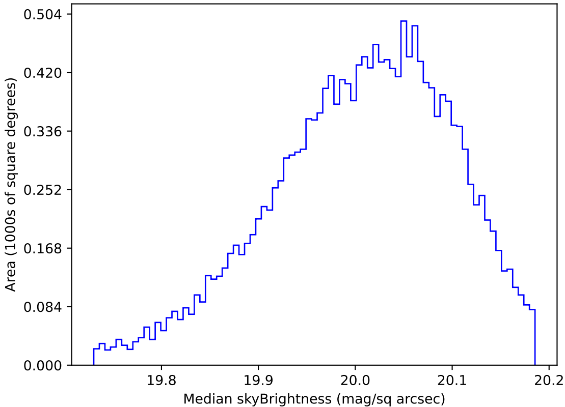
too_elab_r8_d3_griz_v3.4_10yrs WFD i band: Median skyBrightness
