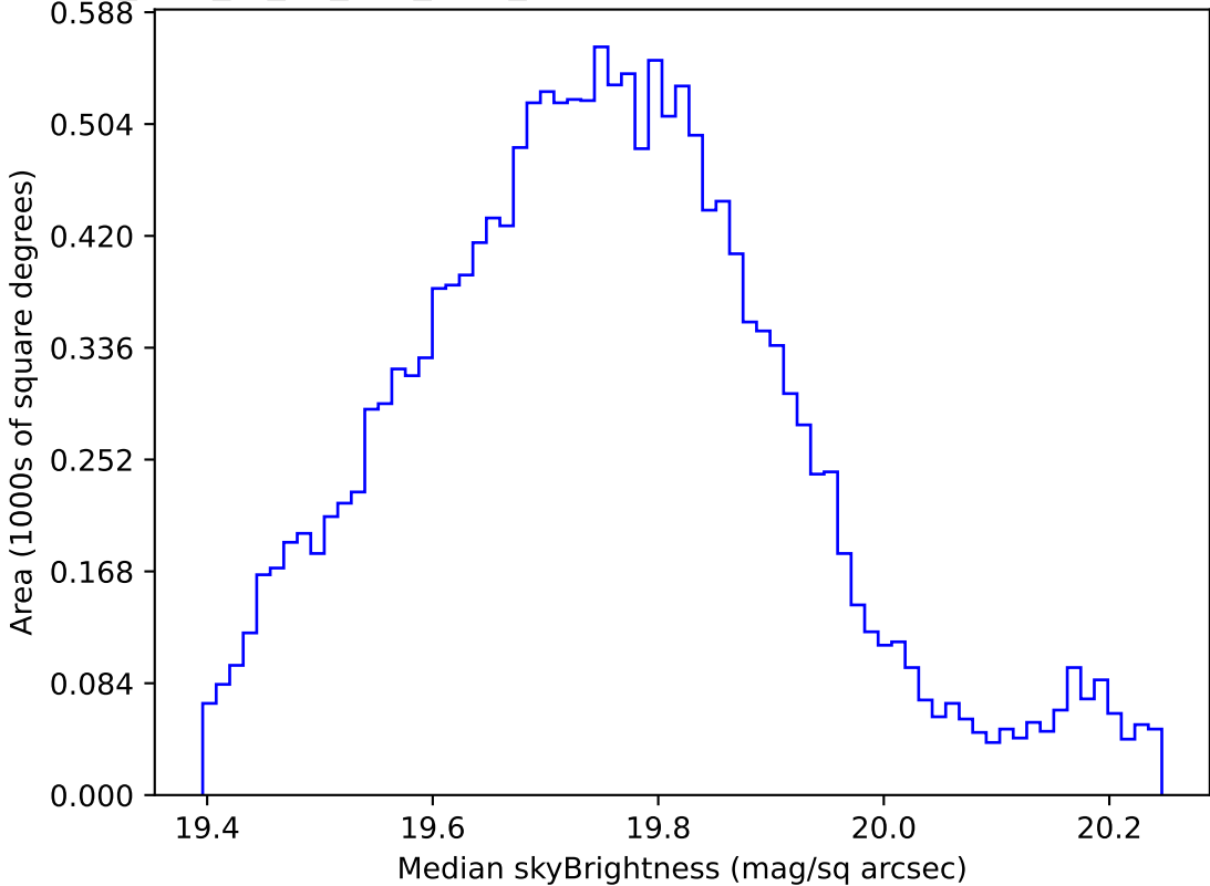
too_elab_r8_d3_griz_v3.4_10yrs WFD all bands: Median skyBrightness
