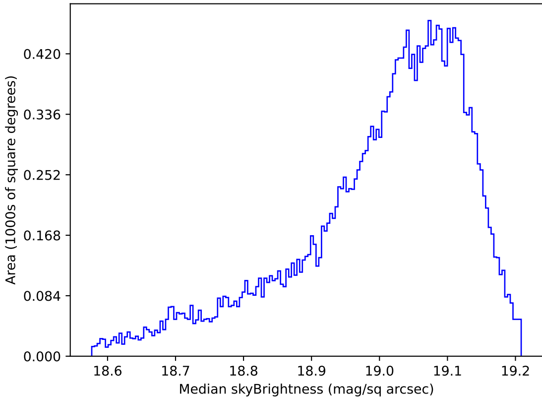
too_elab_r8_d3_griz_v3.4_10yrs All sky z band: Median skyBrightness
