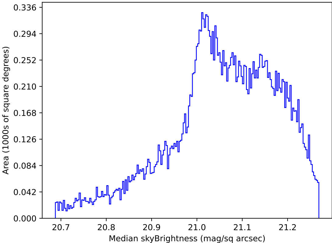
too_elab_r8_d3_griz_v3.4_10yrs All sky r band: Median skyBrightness
