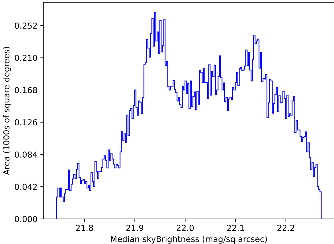
too_elab_r8_d3_griz_v3.4_10yrs All sky g band: Median skyBrightness
