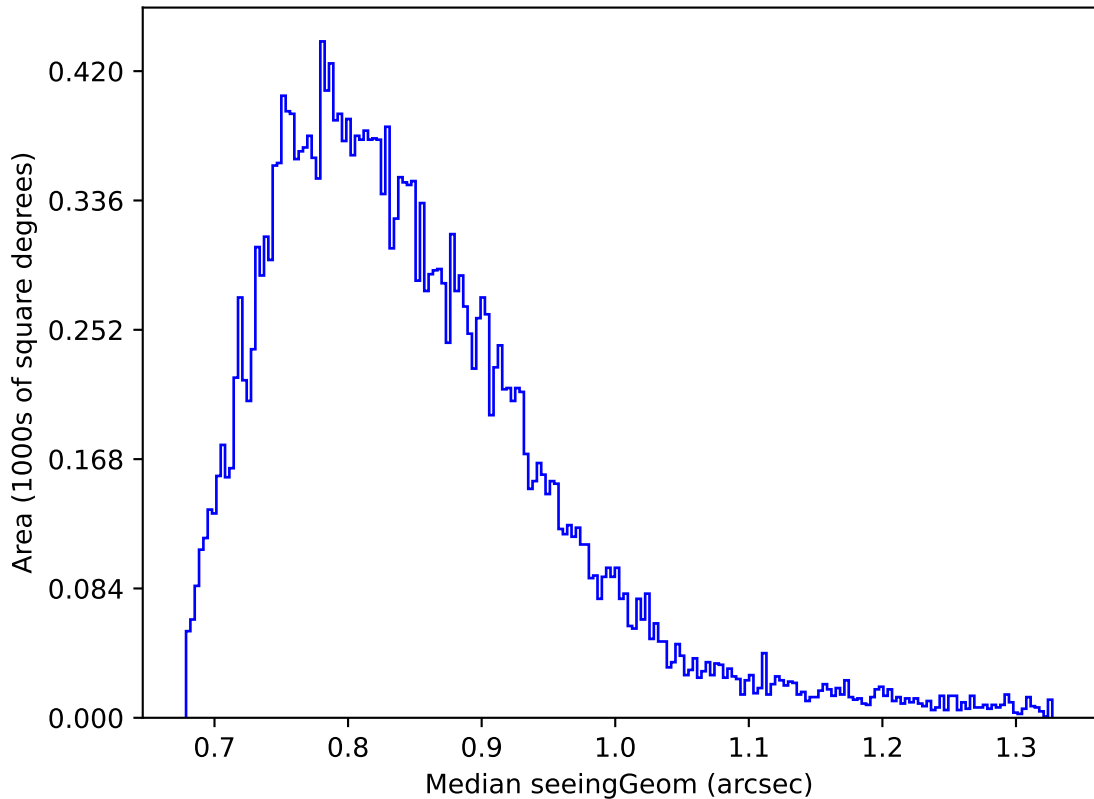
too_elab_r8_d3_griz_v3.4_10yrs Yr 1 z band: Median seeingGeom
