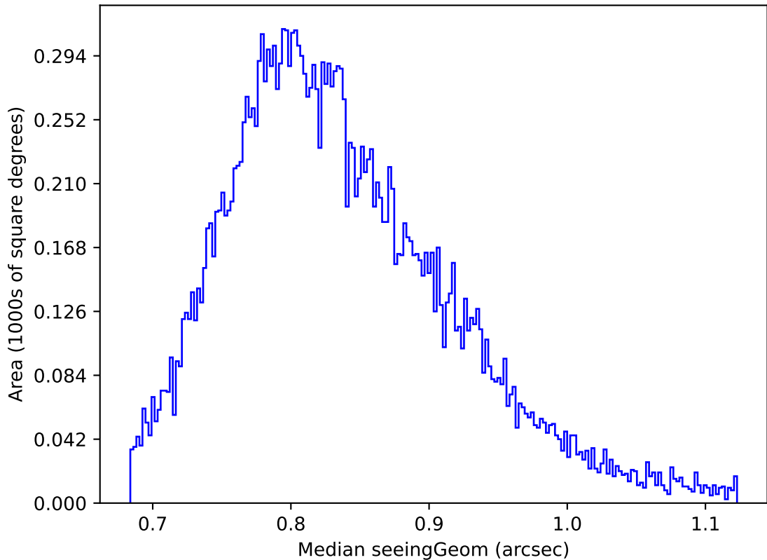
too_elab_r8_d3_griz_v3.4_10yrs Yr 1 y band: Median seeingGeom
