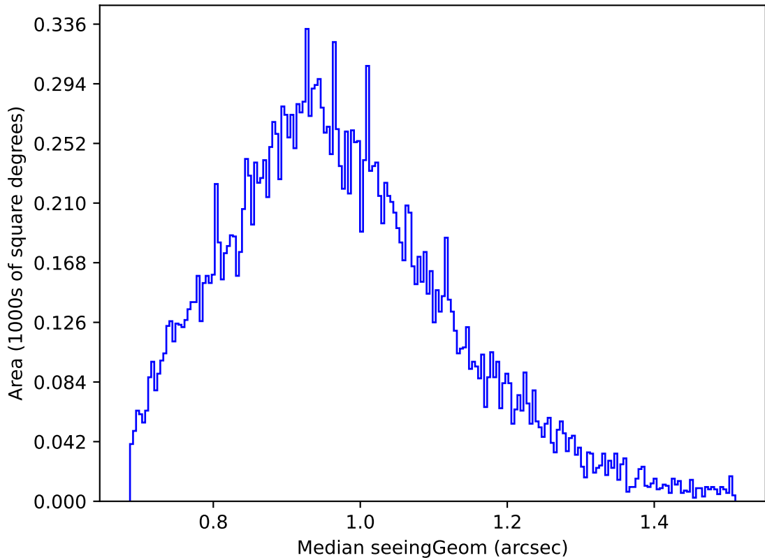
too_elab_r8_d3_griz_v3.4_10yrs Yr 1 u band: Median seeingGeom
