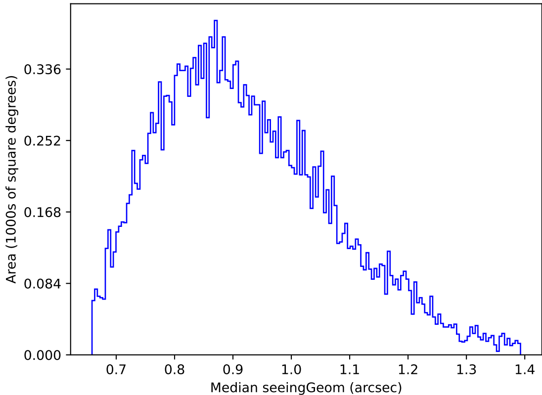
too_elab_r8_d3_griz_v3.4_10yrs Yr 1 g band: Median seeingGeom
