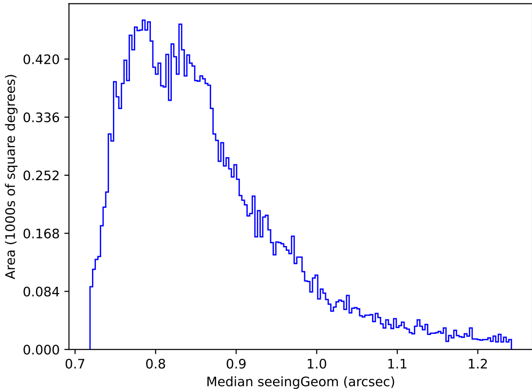
too_elab_r8_d3_griz_v3.4_10yrs Yr 1 all bands: Median seeingGeom
