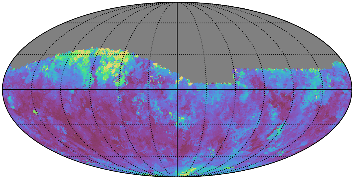
too_elab_r8_d3_griz_v3.4_10yrs Yr 1 z band: Median seeingEff
