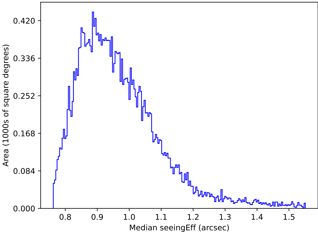
too_elab_r8_d3_griz_v3.4_10yrs Yr 1 z band: Median seeingEff
