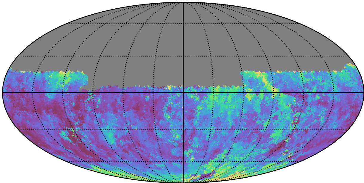
too_elab_r8_d3_griz_v3.4_10yrs Yr 1 y band: Median seeingEff
