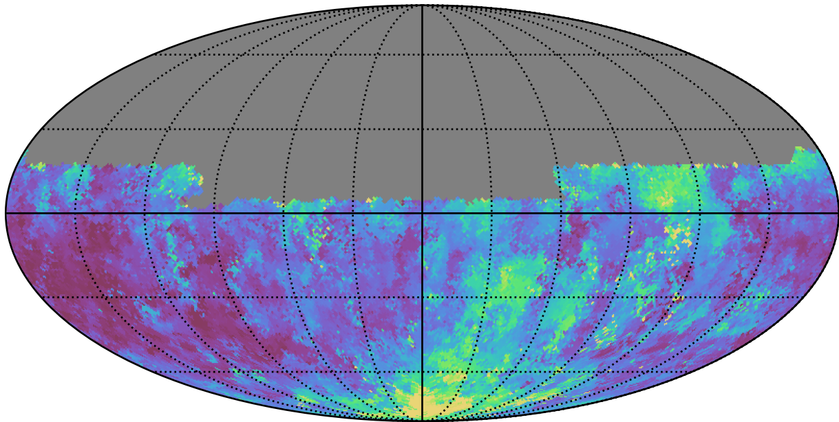
too_elab_r8_d3_griz_v3.4_10yrs Yr 1 u band: Median seeingEff
