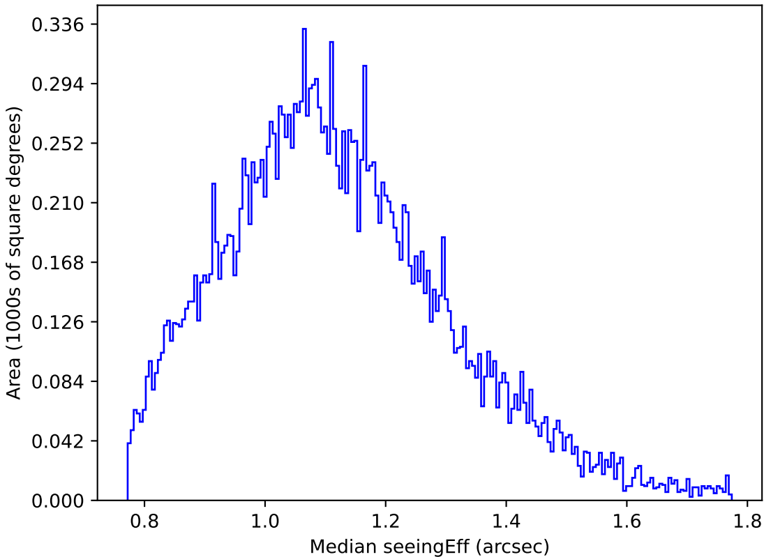
too_elab_r8_d3_griz_v3.4_10yrs Yr 1 u band: Median seeingEff
