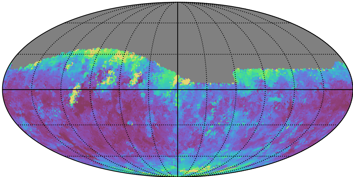
too_elab_r8_d3_griz_v3.4_10yrs Yr 1 r band: Median seeingEff
