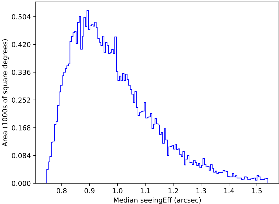
too_elab_r8_d3_griz_v3.4_10yrs Yr 1 r band: Median seeingEff
