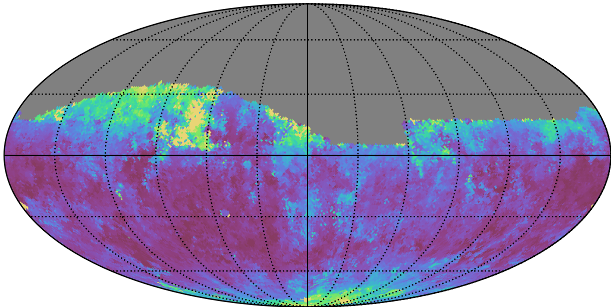
too_elab_r8_d3_griz_v3.4_10yrs Yr 1 i band: Median seeingEff
