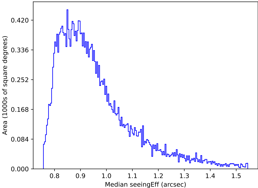
too_elab_r8_d3_griz_v3.4_10yrs Yr 1 i band: Median seeingEff
