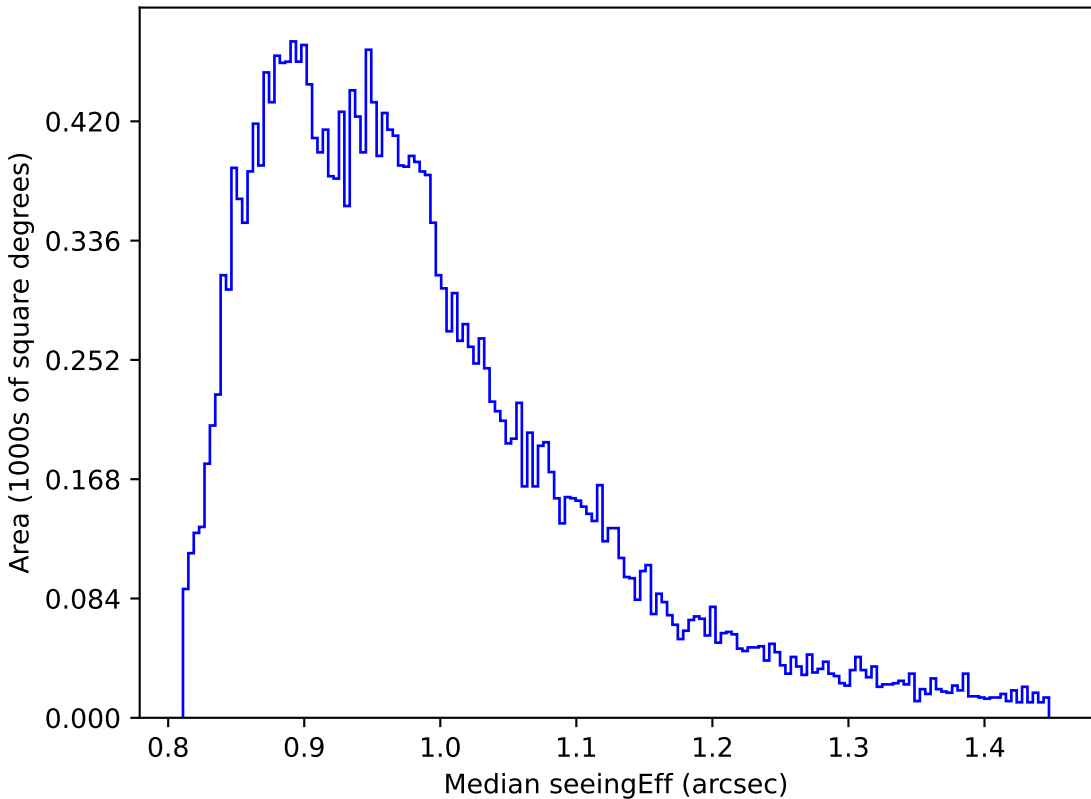
too_elab_r8_d3_griz_v3.4_10yrs Yr 1 all bands: Median seeingEff
