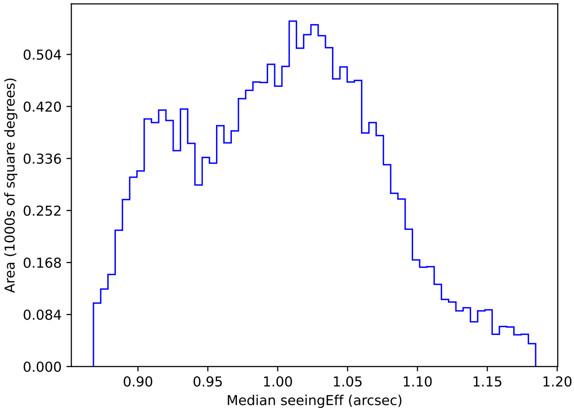
too_elab_r8_d3_griz_v3.4_10yrs WFD z band: Median seeingEff
