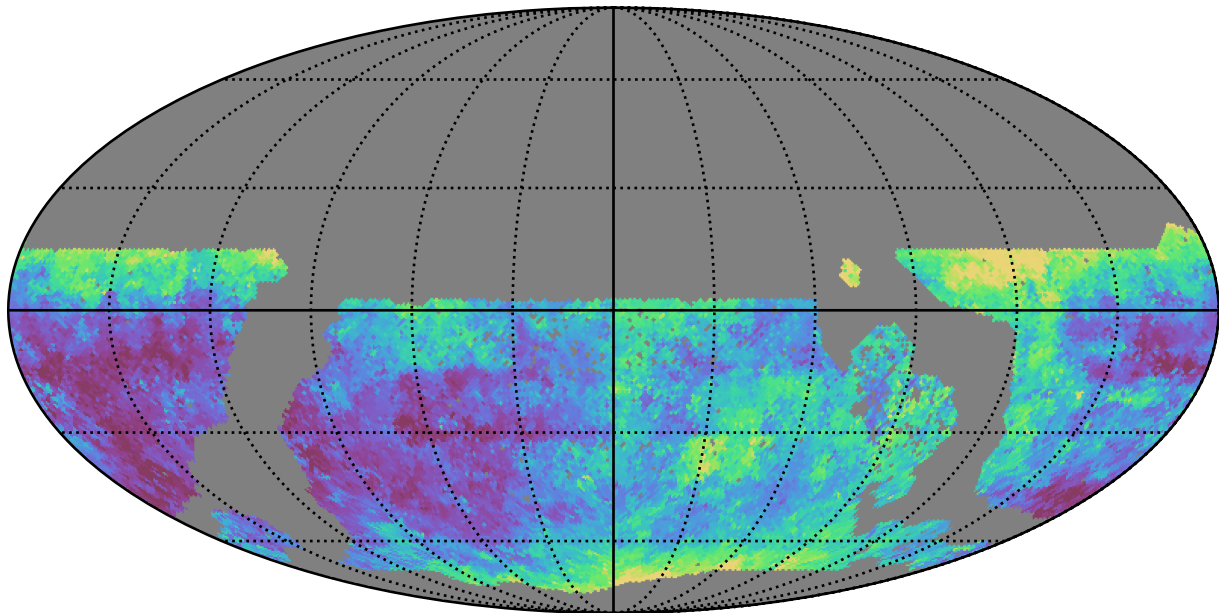
too_elab_r8_d3_griz_v3.4_10yrs WFD u band: Median seeingEff
