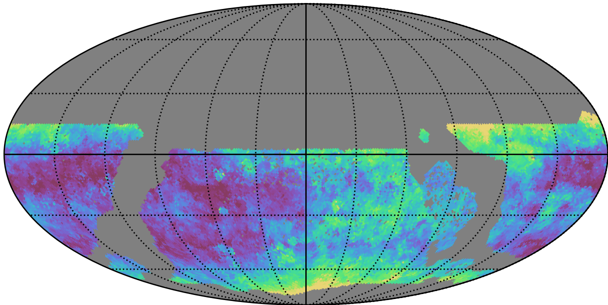
too_elab_r8_d3_griz_v3.4_10yrs WFD g band: Median seeingEff
