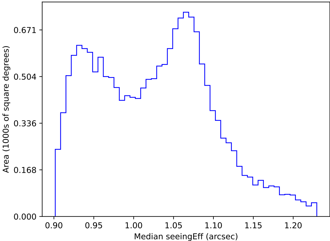
too_elab_r8_d3_griz_v3.4_10yrs WFD all bands: Median seeingEff
