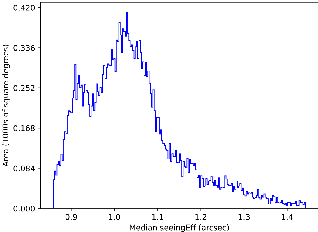
too_elab_r8_d3_griz_v3.4_10yrs All sky z band: Median seeingEff
