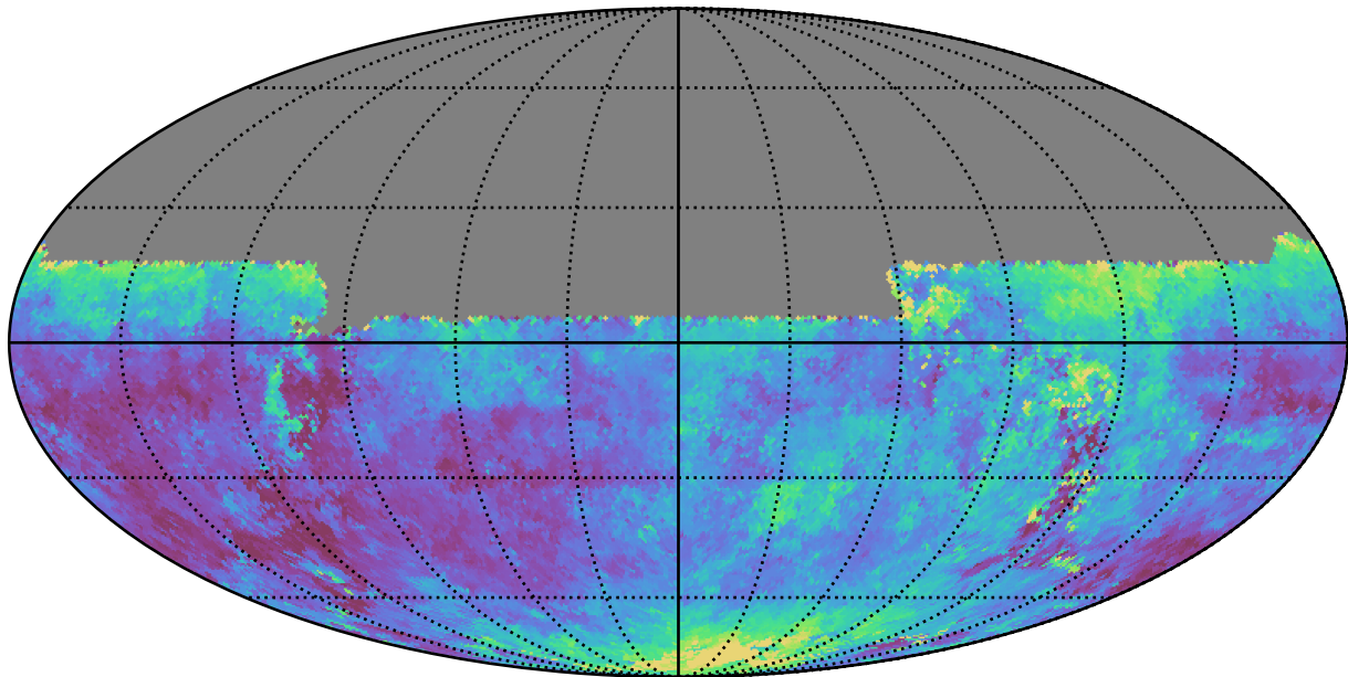
too_elab_r8_d3_griz_v3.4_10yrs All sky u band: Median seeingEff
