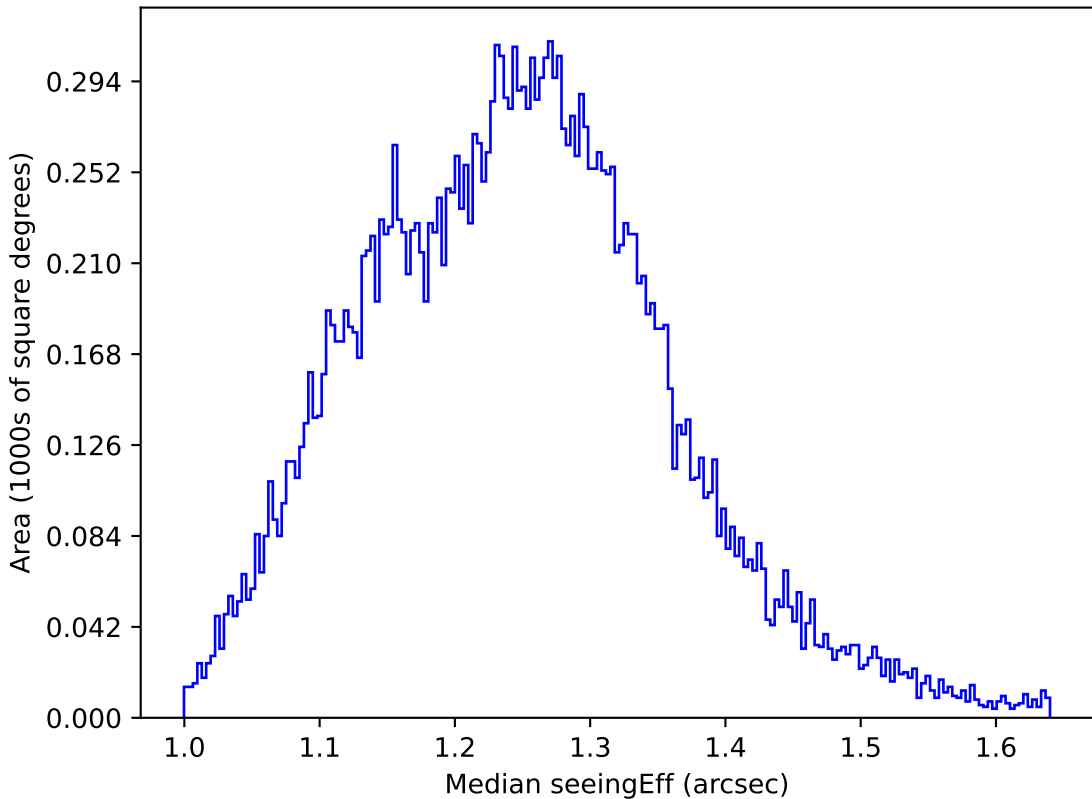
too_elab_r8_d3_griz_v3.4_10yrs All sky u band: Median seeingEff
